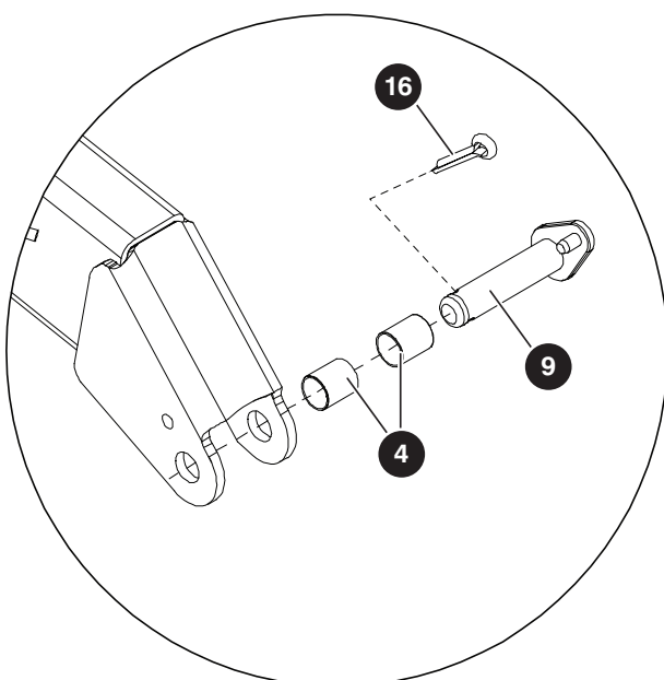
Bottom End Pin Assembly
