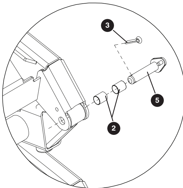
Inside End Pin Assembly (Without Cross Member Tube)
