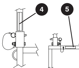
RAILING PINS
