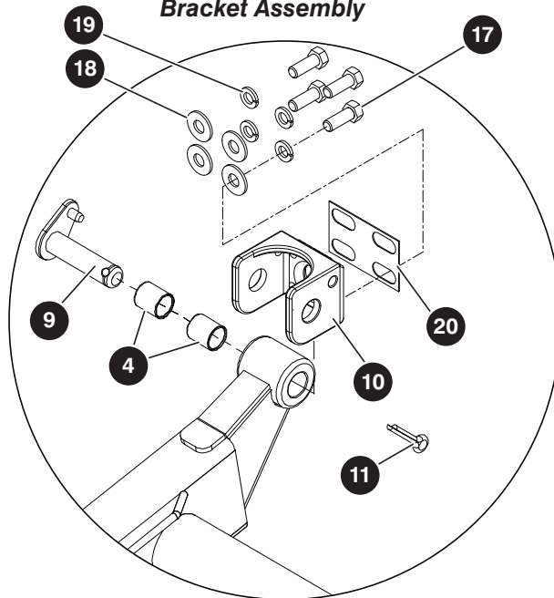
Platform Mounting Bracket Assembly
