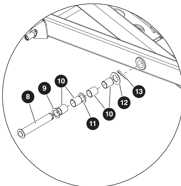
Center Pin Assembly
